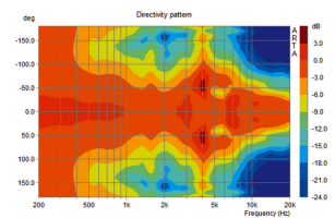
ESP-250WS Directivity horizontal
