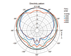
ESP-250WS Directivity horizontal
